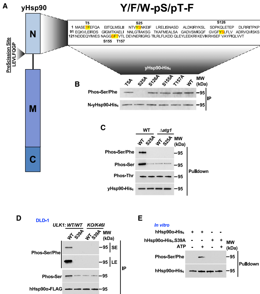
Figure 1. Ulk1-mediated phosphorylation of a conserved serine in amino domain of Hsp90
