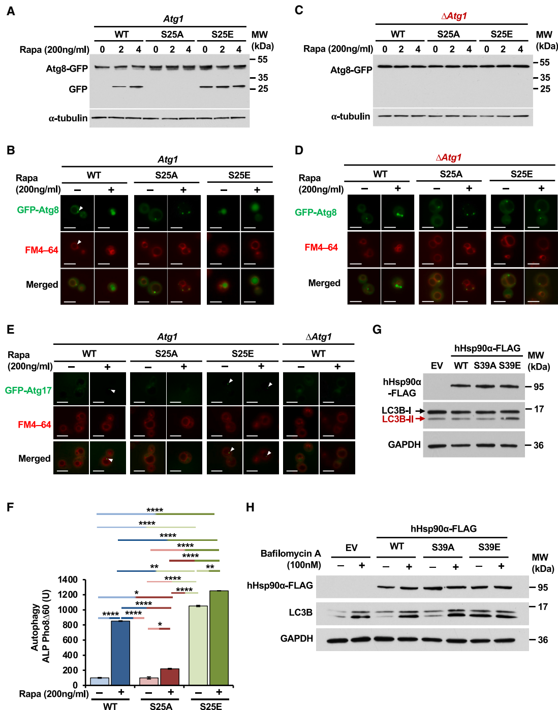
Figure 5. Atg1/Ulk1-mediated phosphorylation of Hsp90 is essential for autophagy induction
