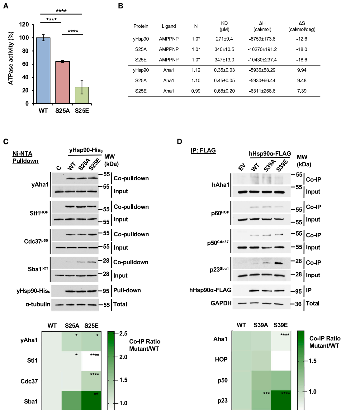
Figure 2. Phosphorylation of S25/S39 affects Hsp90 ATPase activity and co-chaperone binding
